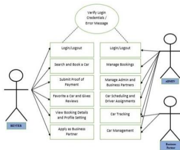
Figure 3: Use Case Diagram
