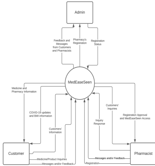
Figure 6: Context Diagram
