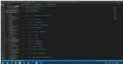
Figure 5: Visual Studio
