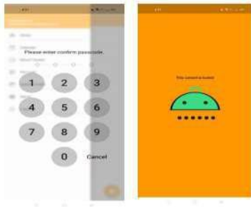
Figure 10. Pin Code
