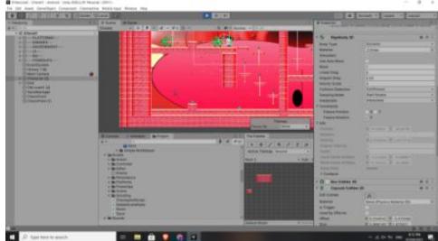
Figure 11: Collision Detection
