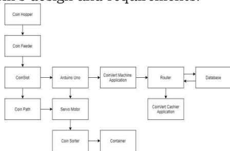
Figure 2: Block Diagram
