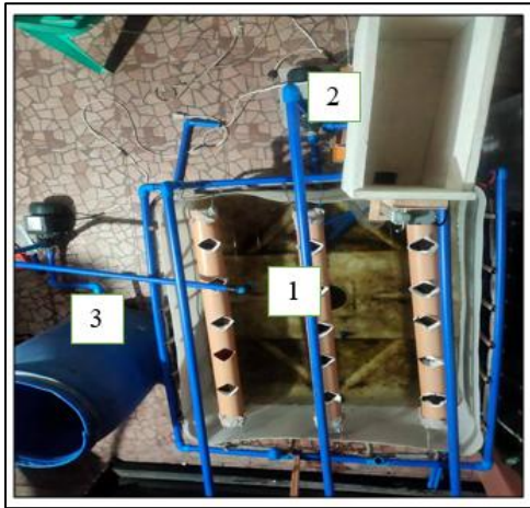
Figure 9. Top View 1- Aquaponics system, 2 – feeding system, 3 – water system
