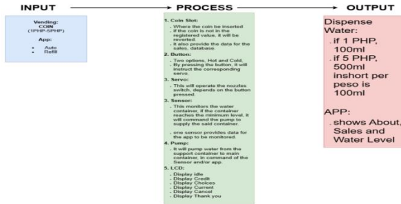
Figure 5: Block Diagram
