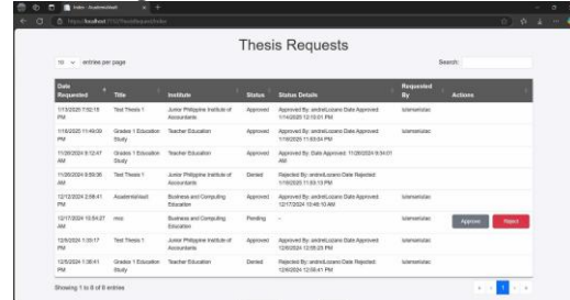
Figure 8: Thesis Request in Library Account
